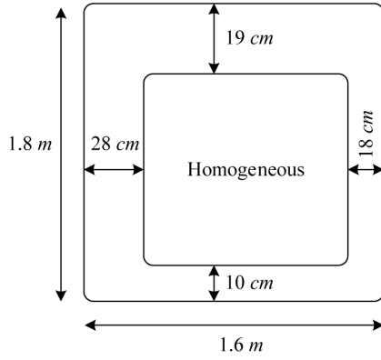
FIG. 2. Homogeneity within the chamber.
