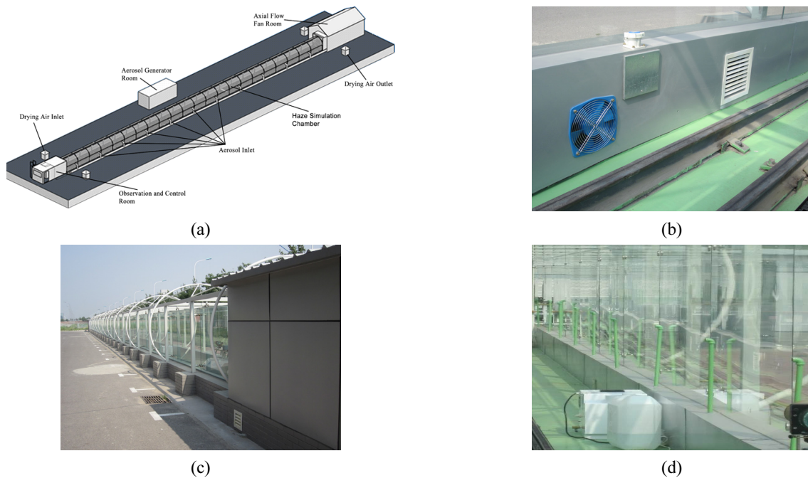
FIG. 1. (a) Schematic diagram of the atmospheric environment simulation chamber; (b) A horizontal fan and ventilation duct pair; (c) Photo of atmospheric environment simulation chamber; (d) The aerosol inlet inside the chamber.
